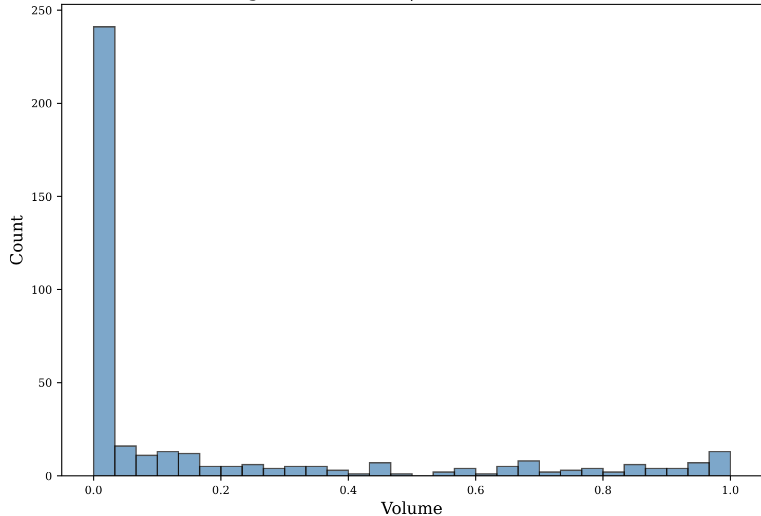
Volume Distribution of Downsampled Sequences (Filtered >20 seqs per motif) sigma: (0.02, 0.4) | volume: (0.1, 0.5)
